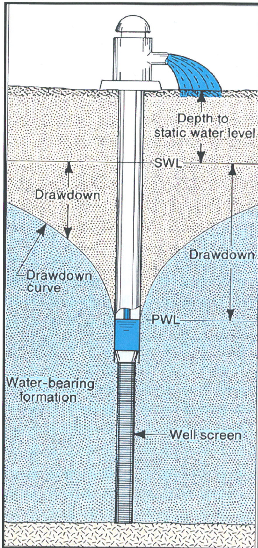
Drawdown Due To Pumping
