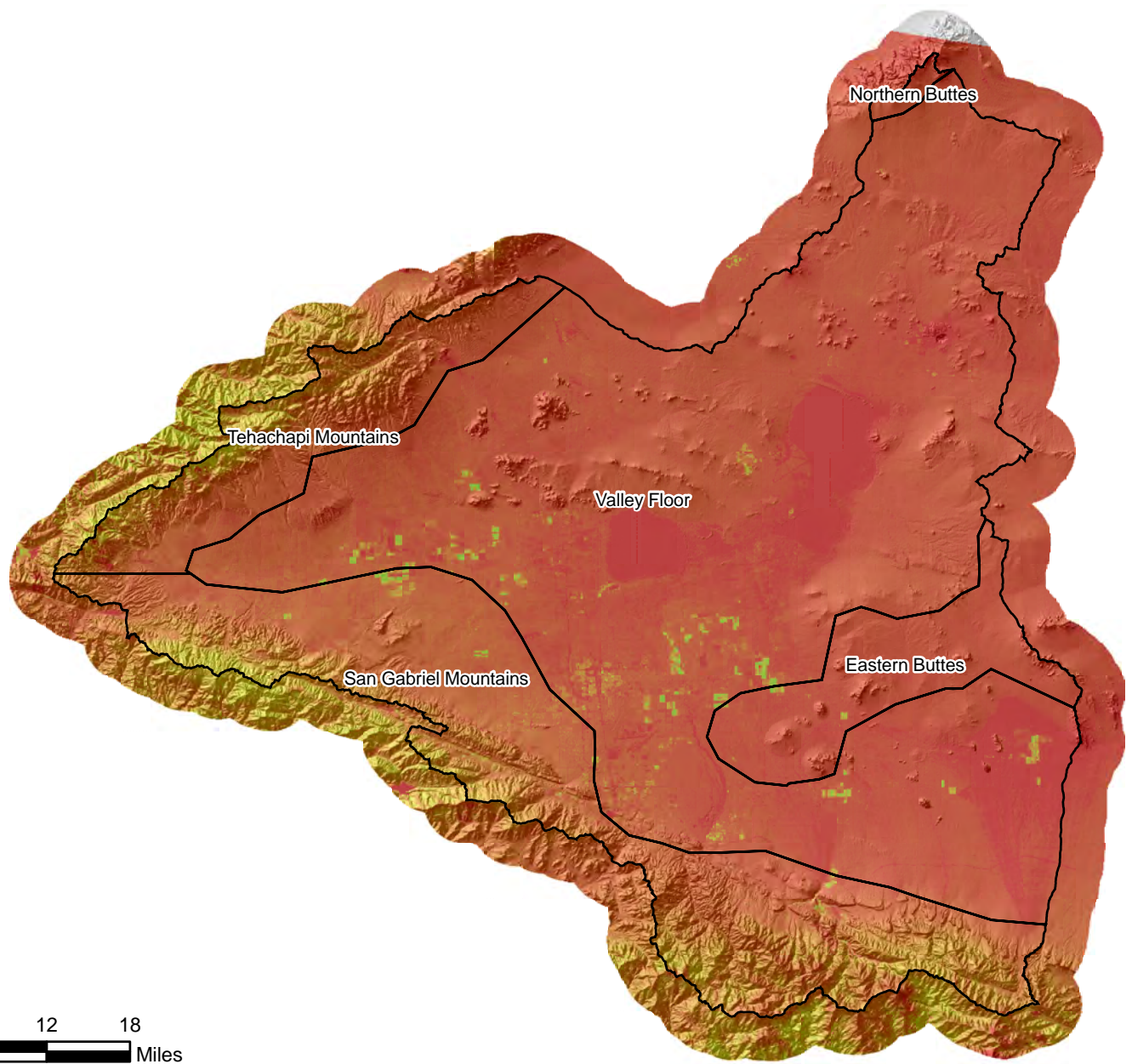
Figure C.26d Geographic Distribution of ET for June 1986
