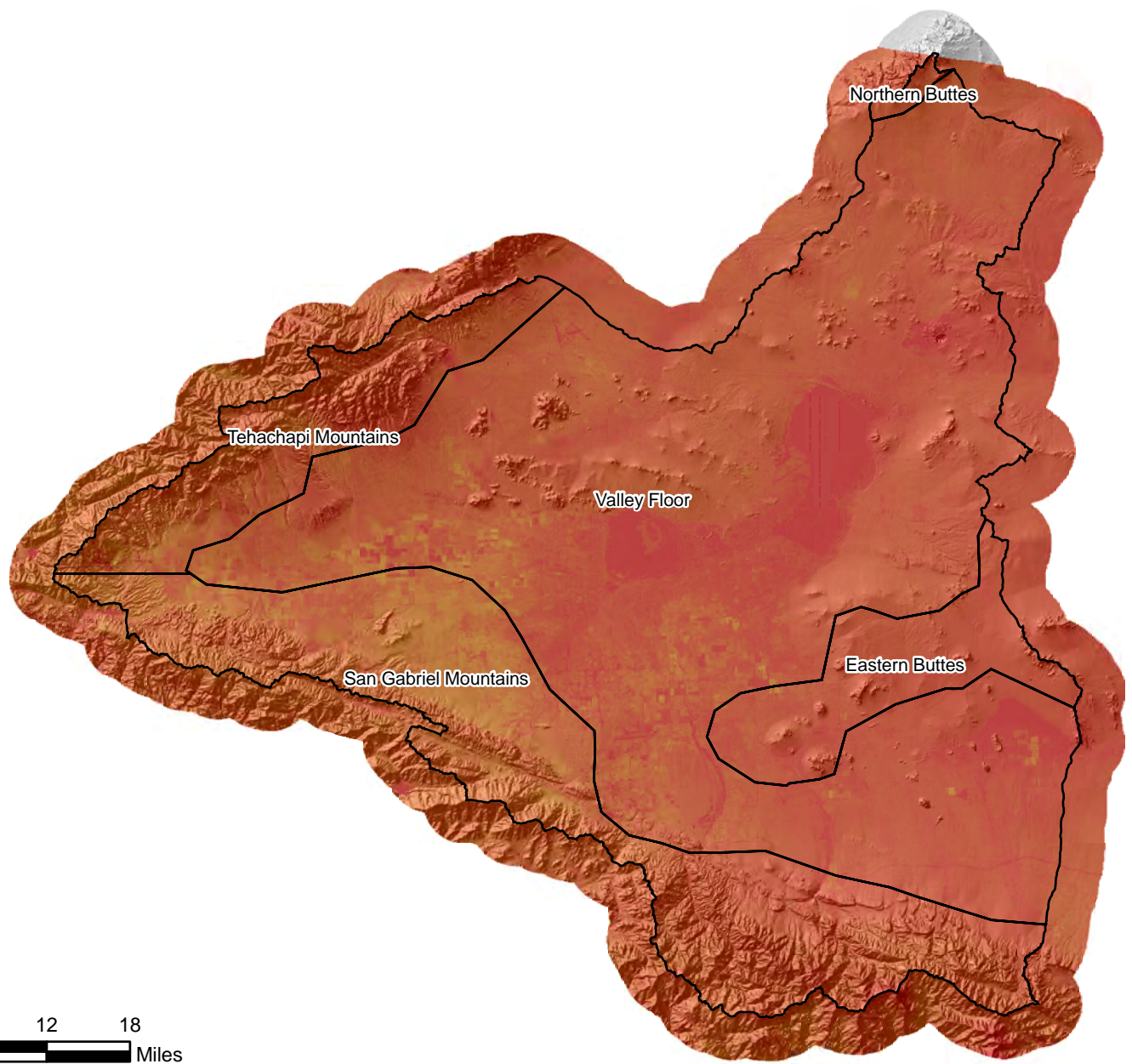
Figure C.26c Geographic Distribution of ET for February 1986
