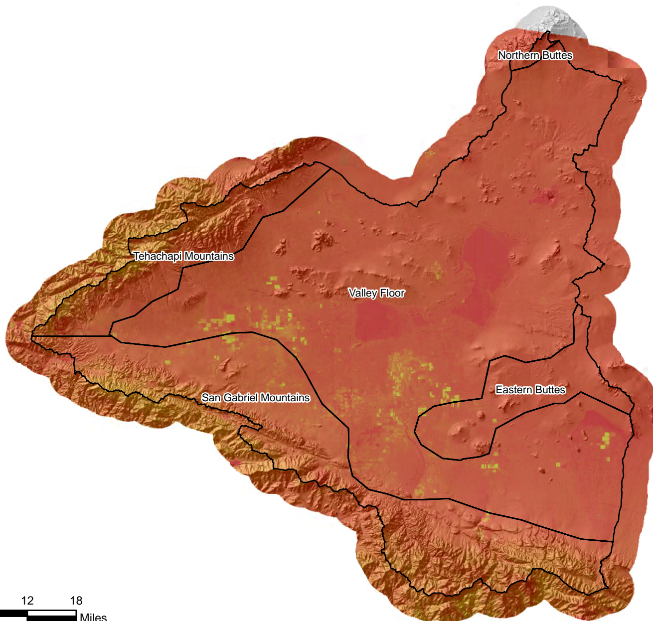
Figure C.26a Geographic Distribution of ET for September 1985
