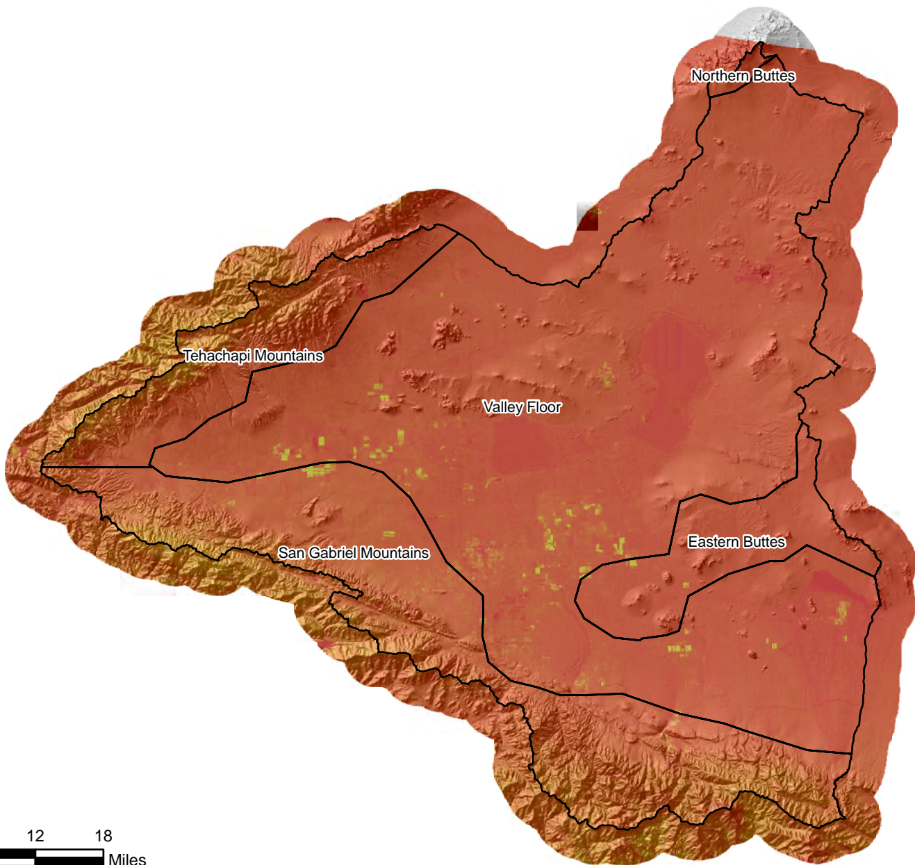
Figure C.26f Geographic Distribution of ET for September 1986
