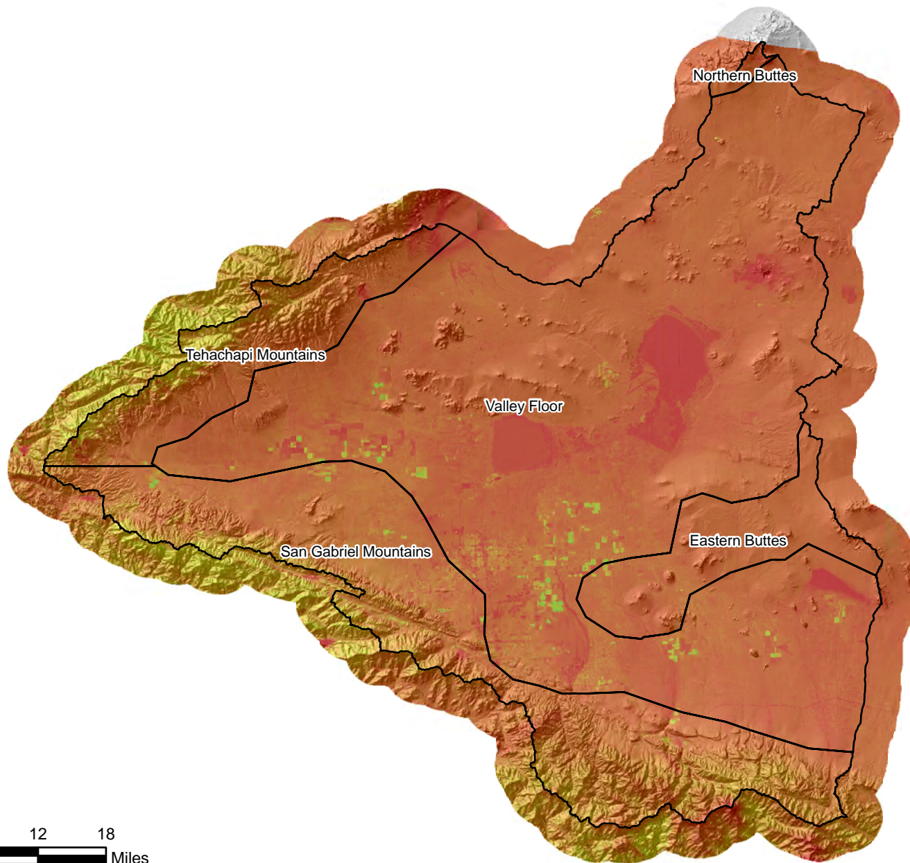
Figure C.26j Geographic Distribution of ET for June 2005
