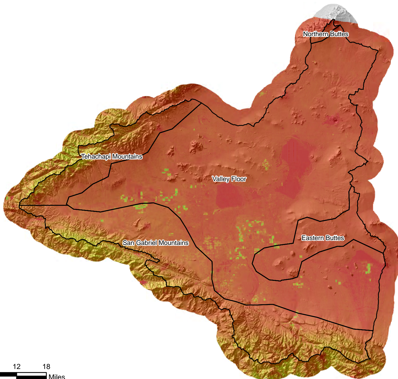
Figure C.26e Geographic Distribution of ET for August 1986
