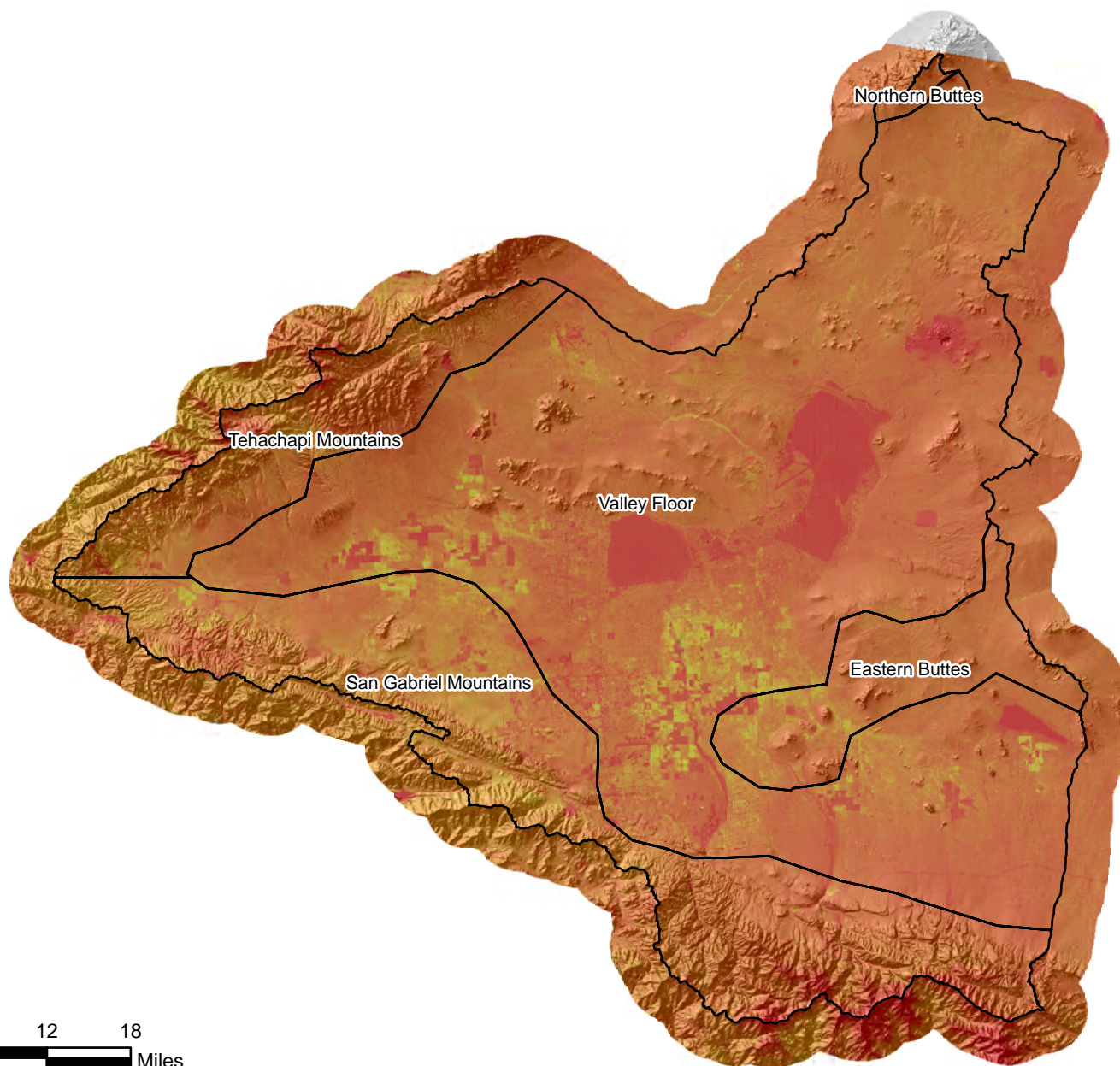
Figure C.26i Geographic Distribution of ET for April 2005
