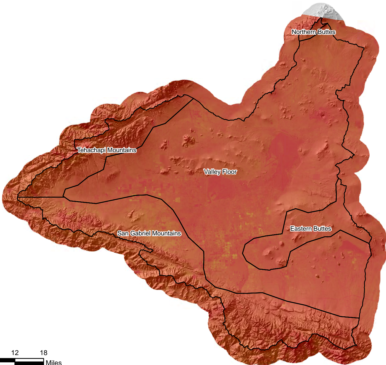
Figure C.26h Geographic Distribution of ET for November 2004
