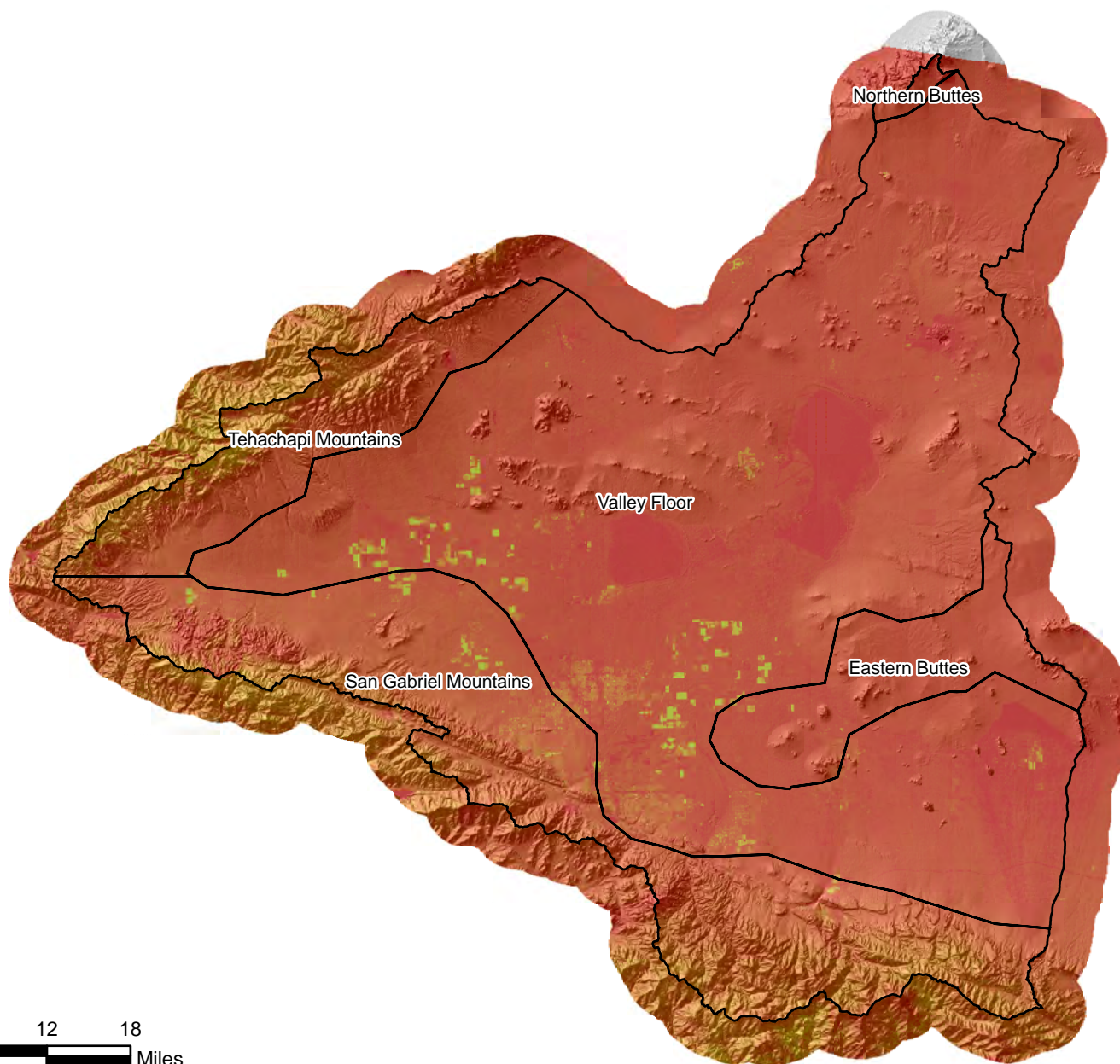
Figure C.26g Geographic Distribution of ET for September 2004
