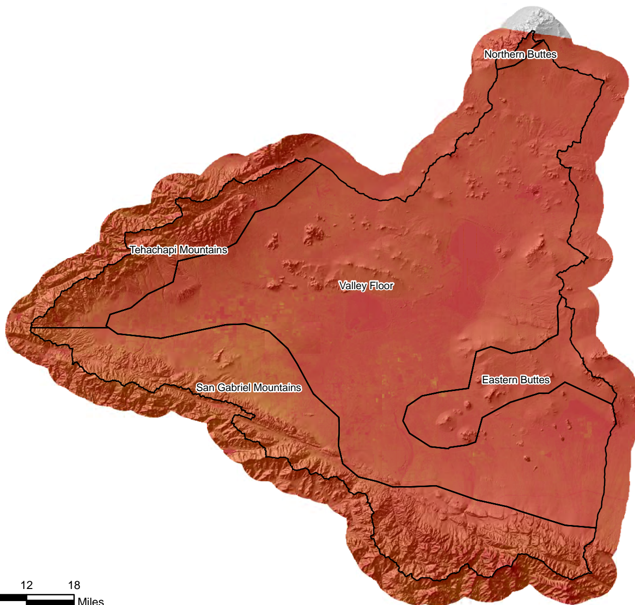
Figure C.26b Geographic Distribution of ET for January 1986
