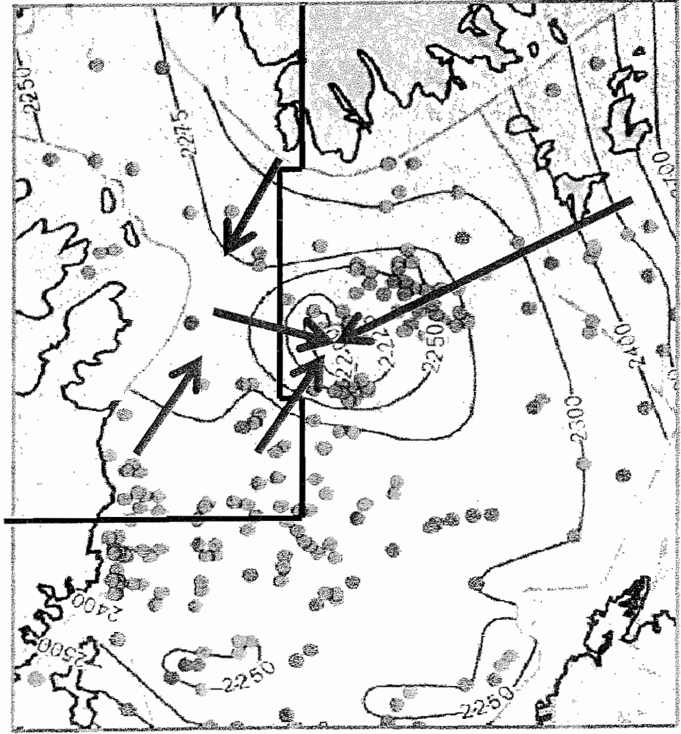
1951 Groundwater Levels, Modified from Wildermuth Exhibit 20, arrows and EAFB boundary added
