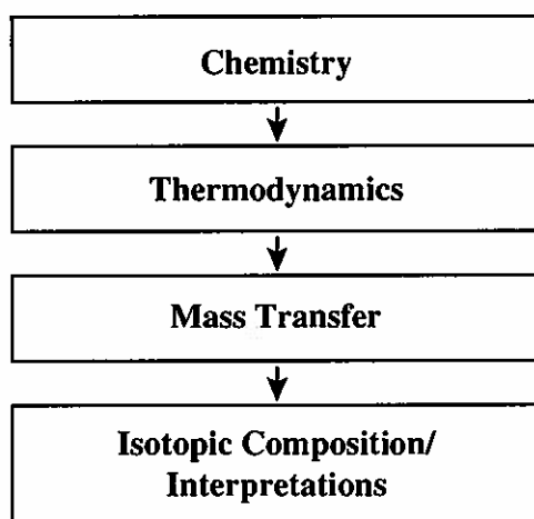
Figure 8. Interpretation of changes in chemistry, thermodynamics, mass transfer, and isotopic composition of water from wells along a flow path.
