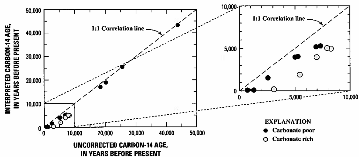
Figure 12. Comparison of uncorrected carbon-14 ages and interpreted carbon-14 ages for ground water in the Mojave River and the Morongo ground-water basins, southern California.
