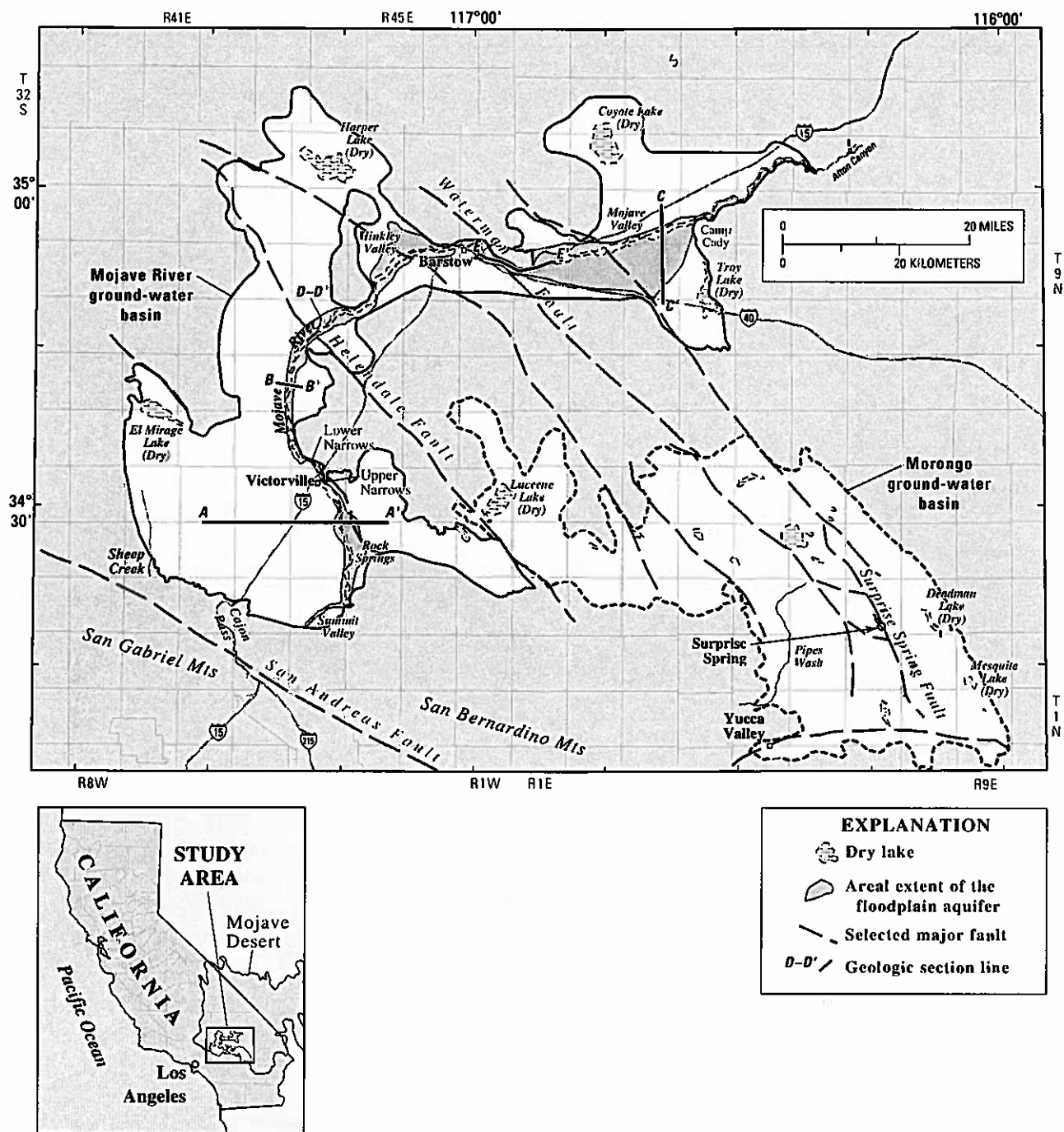
Figure 1. Location of study area, the Mojave River and the Morongo ground-water basins, the floodplain aquifer, selected faults, and geologic section lines.
