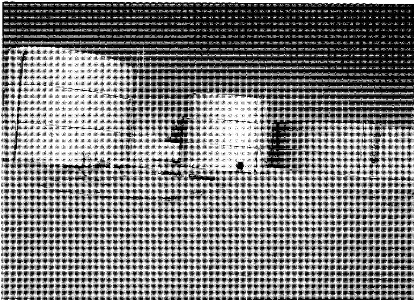
ZONE A 126,000 GAL. STORAGE TANK + 500,000 GAL. TANK, CENTER TANK NOT USED.
