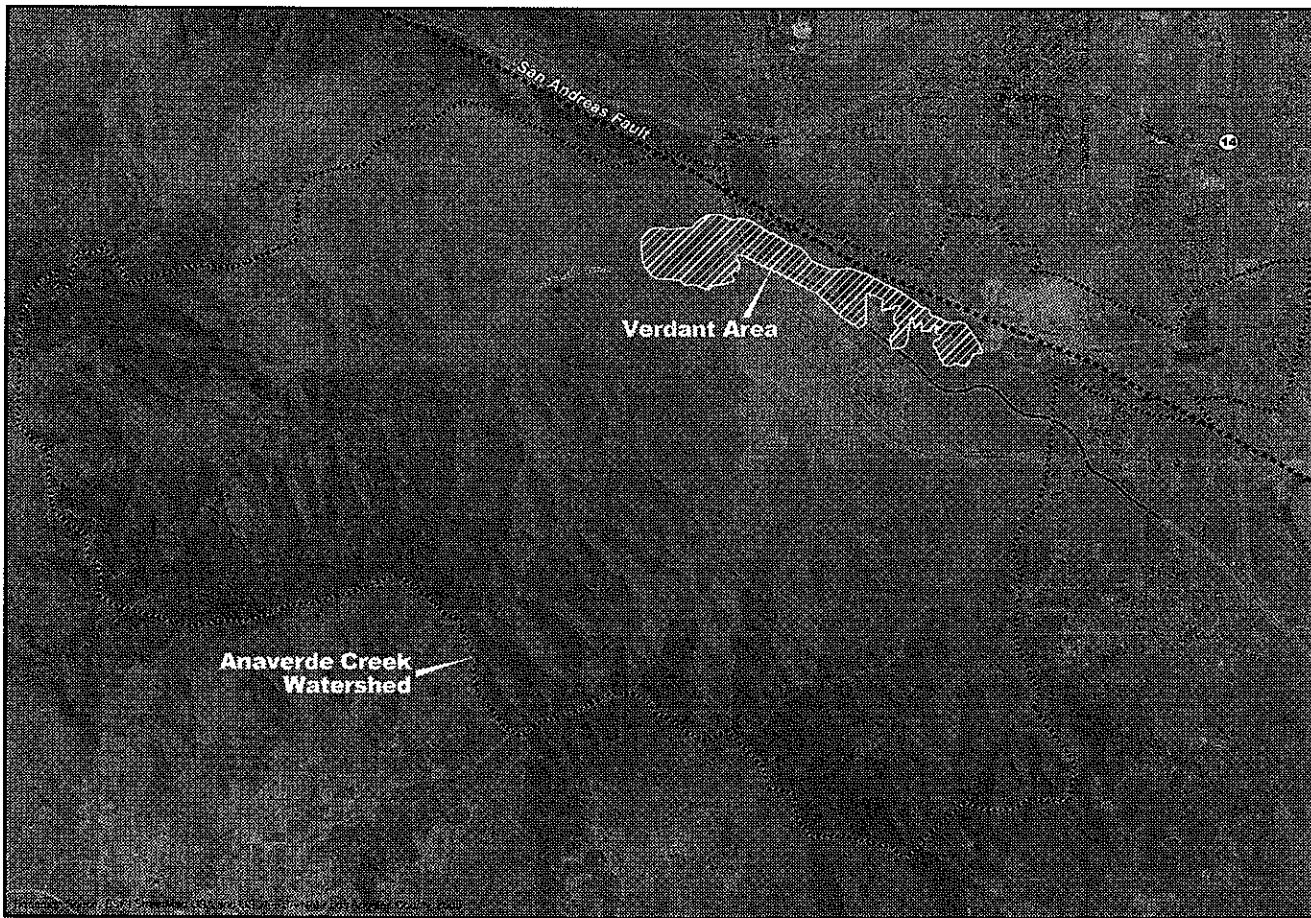
Exhibit 13 Estimated Verdant Area in Anaverde Creek Groundwater Basin
