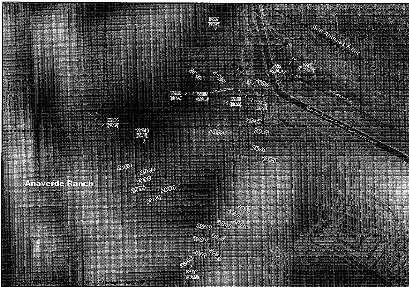
Exhibit 12 Summer 2008 Groundwater Contour Map On Site
