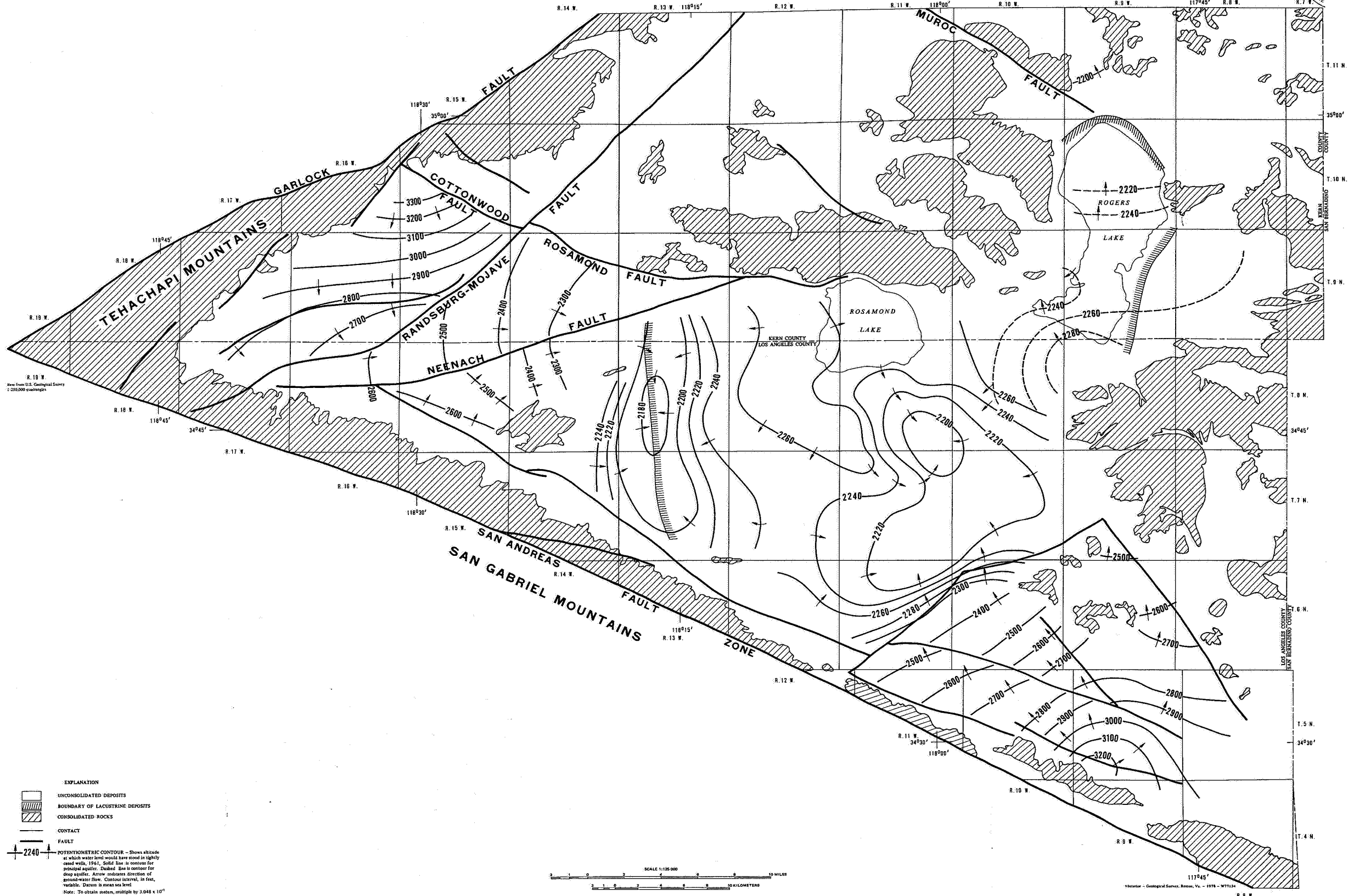
POTENTIOMETRIC MAP FOR 1961, ANTELOPE VALLEY, CALIFORNIA
