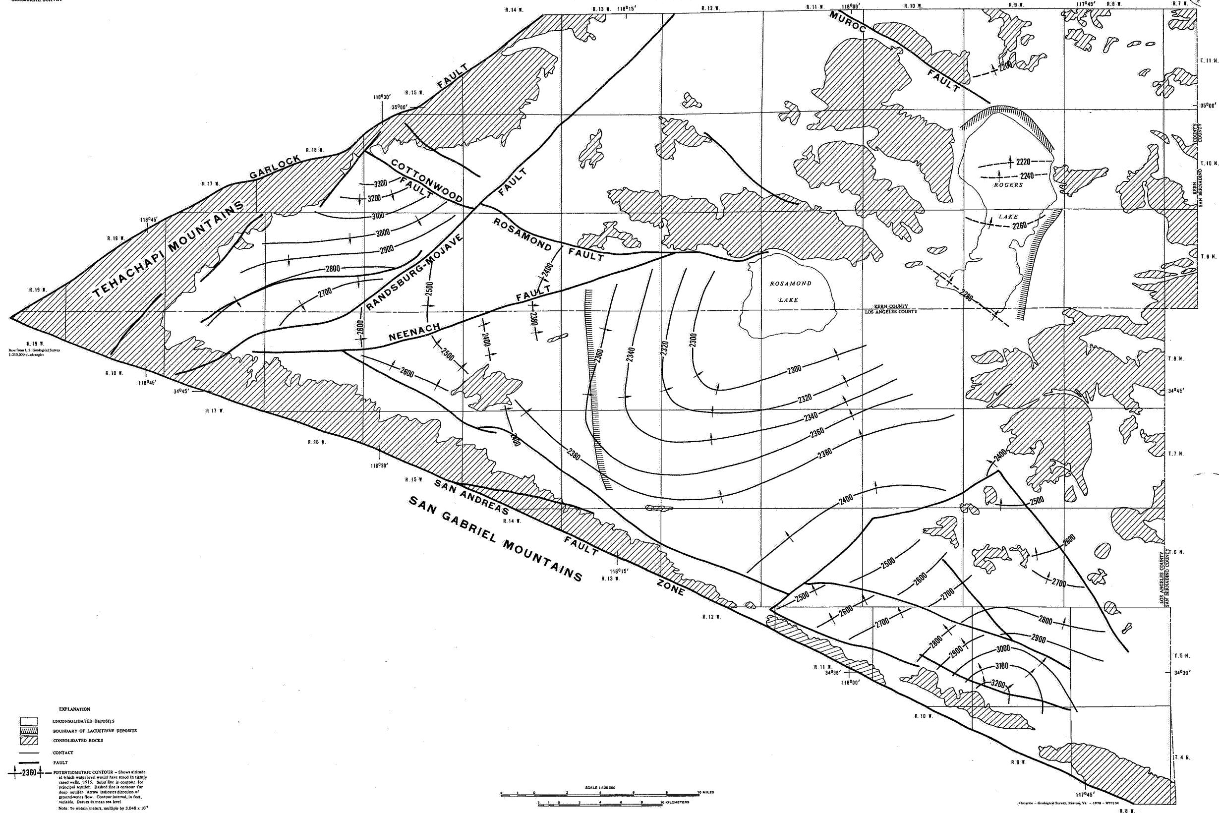
POTENTIOMETRIC MAP FOR 1915, ANTELOPE VALLEY, CALIFORNIA
