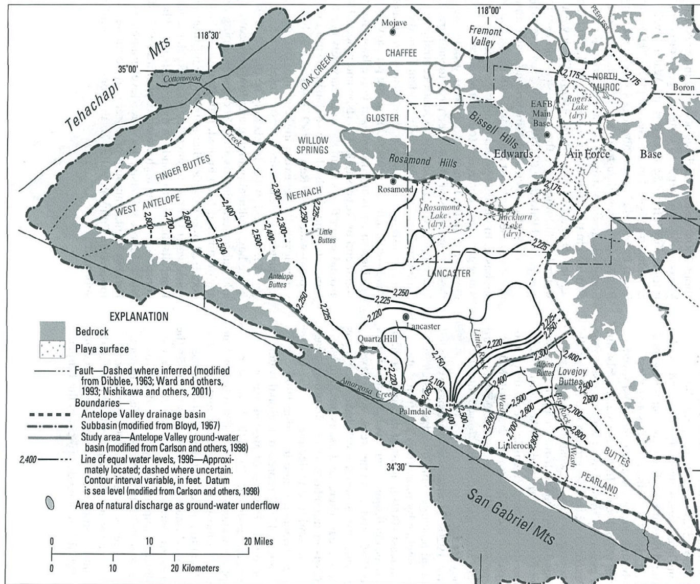
Figure 7. Ground-water levels in spring 1996 and location of area of natural discharge as ground-water underflow in the Antelope Valley ground-water basin, California.
