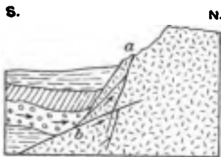
FIGURE 10.—Diagram showing possible origin of Gerblich Spring.
