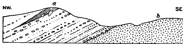
FIGURE 2.—Section of Antelope Buttes, showing attitude of tuffs and lava at a , and their relations to granitic rocks at b .
