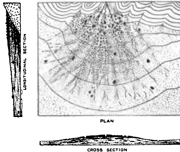
FIGURE 3.—Diagrammatic plan and sections of alluvial fan, showing arrangement of debris. Sketch contours do not show channelling of fan.
