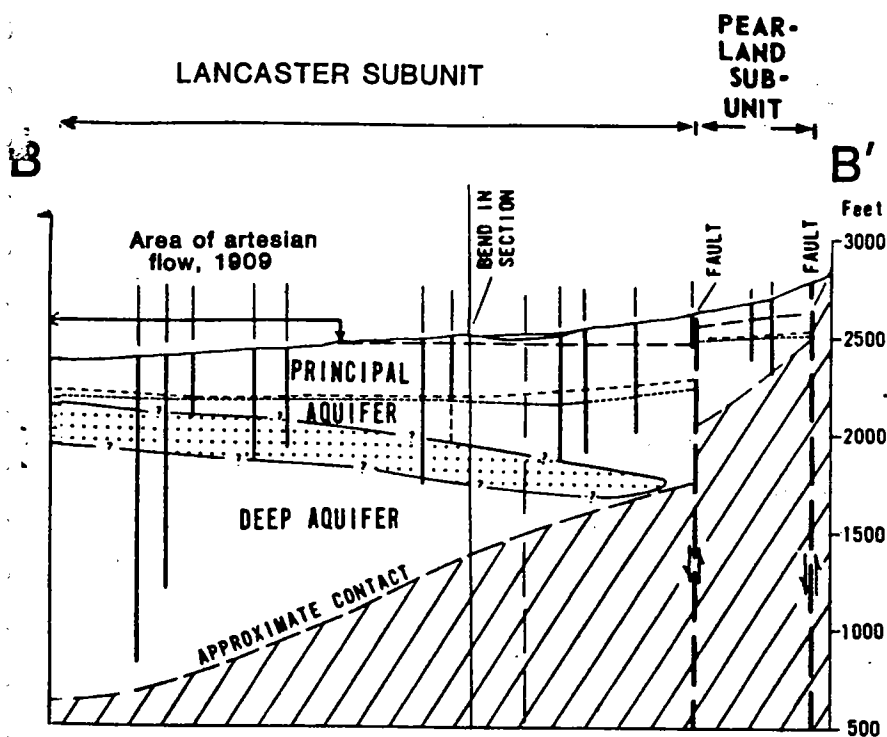
Figure 3 - Generalized geologic cross-section B-B'
