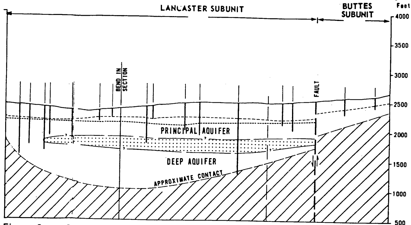
Figure 2 - Generalized geologic cross-section A-A'
