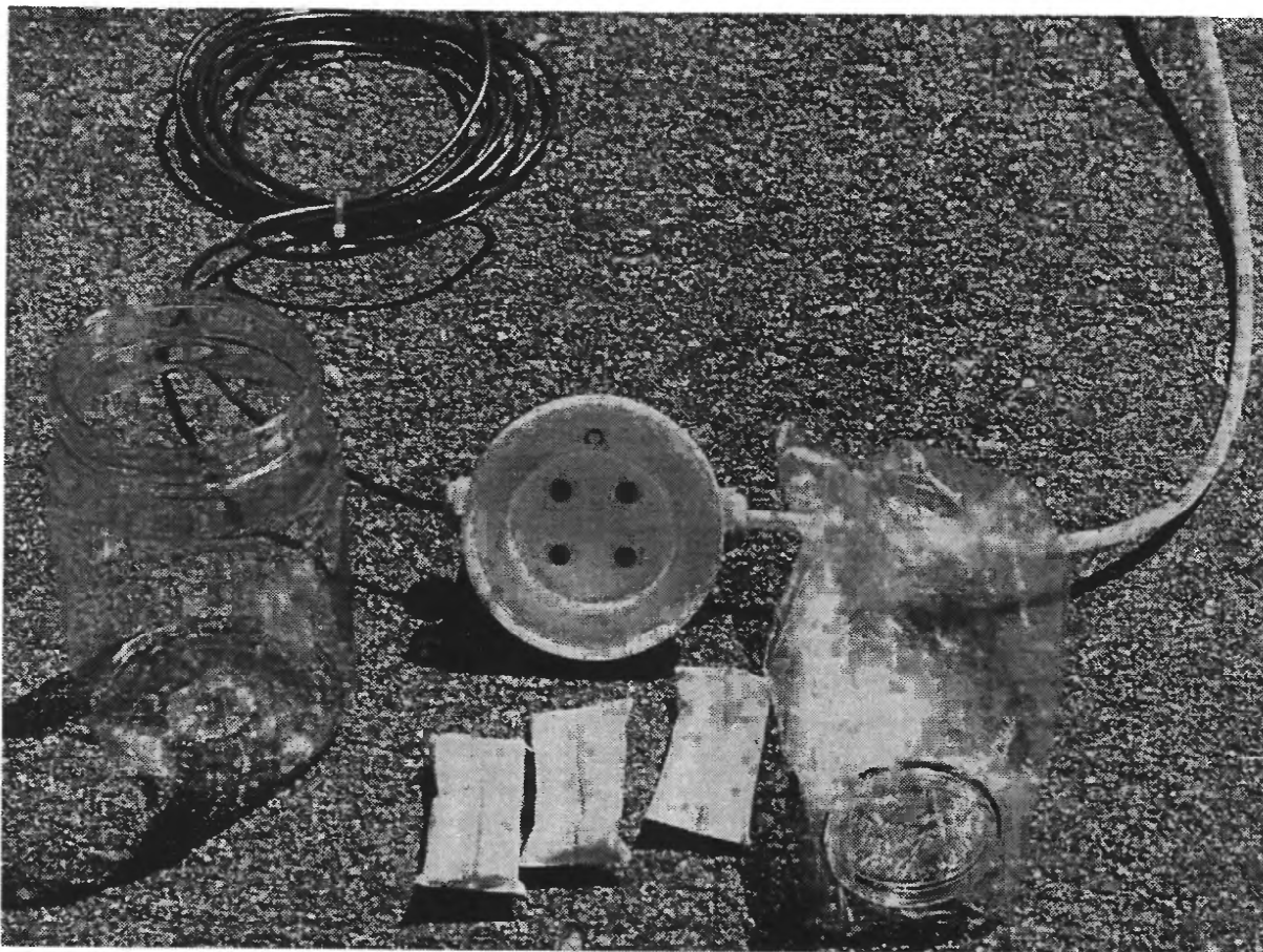
Figure 6. Dry-air system for H-300 submersible pressure transducer (reproduced with permission of Design Analysis, Inc.).
