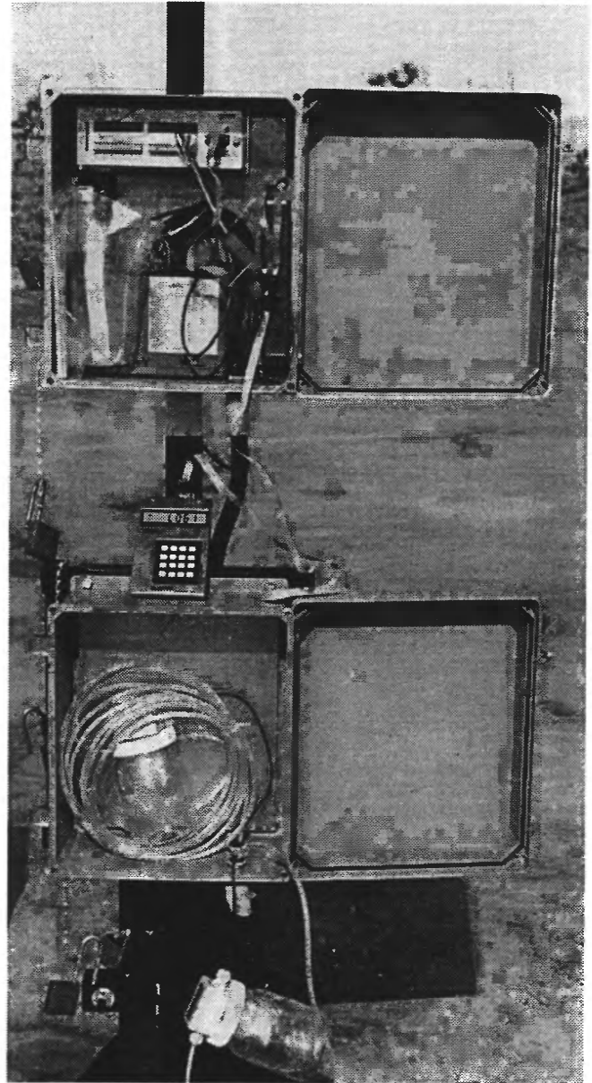
Figure 5. Data logger and transducer system used for recording ground-water levels.
