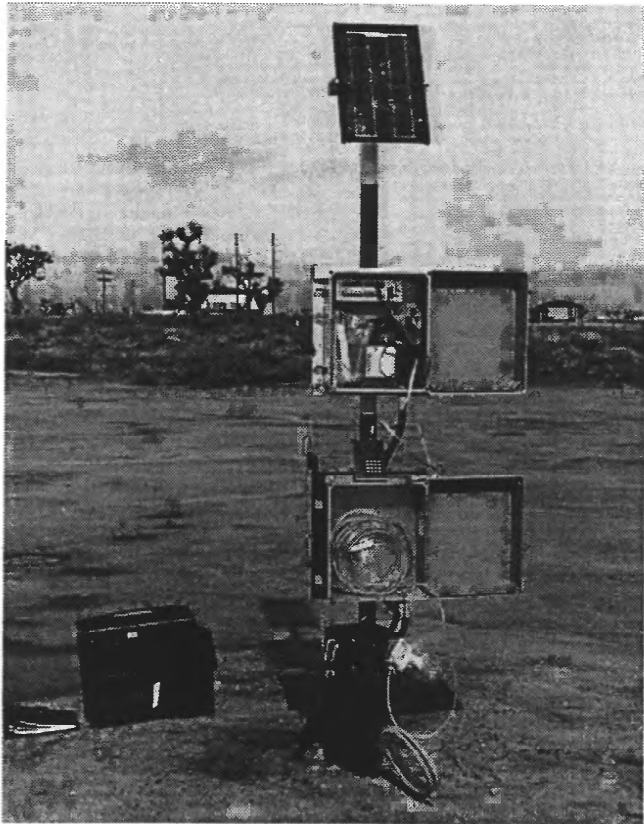
Figure 7. Typical Edwards Air Force Base ground-water level recording site.
