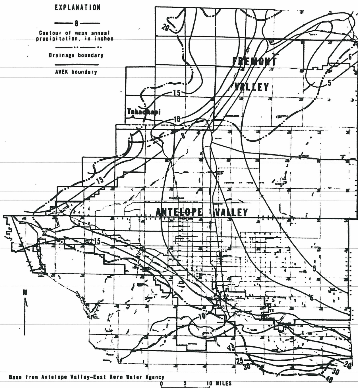
MAP OF THE AVEK AREA SHOWING MEAN ANNUAL PRECIPITATION AND DRAINAGE BOUNDARIES
