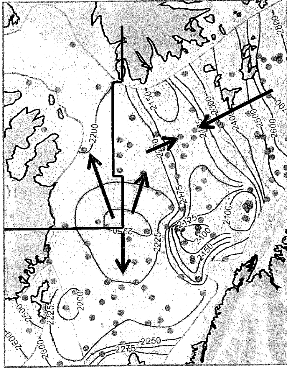
2009 Groundwater Levels, Modified from Wildermuth Exhibit 28, arrows and EAFB boundary added
